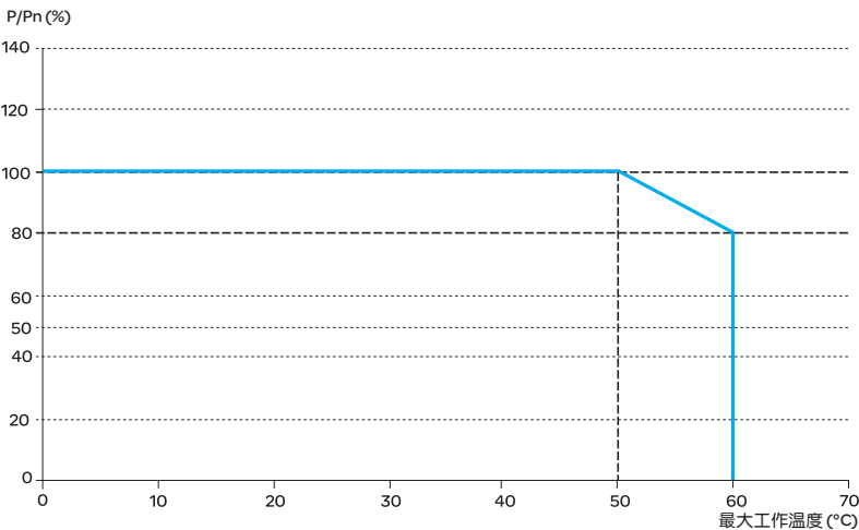
ABL 8RPM, ABL 8RPS, ABL 8WPS，垂直安装
