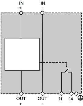
ABL 8BUF24400 缓冲模块
